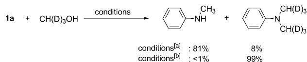
Scheme 3. N -alkylation of 1a using either CH 3 OH or CD 3 OH. Reaction conditions: [a] 1a /CH 3 OH/ FeBr 3 / 4a / Cp*H =250:100:5:10:10, in 1,2,4-TMB at 200 °C for 36 h; [b] 1a /CD 3 OH/ FeBr 3 / 4a / Cp*H =100:266:5:10:10, in 1,2,4-TMB at 200 °C for 36 h.
